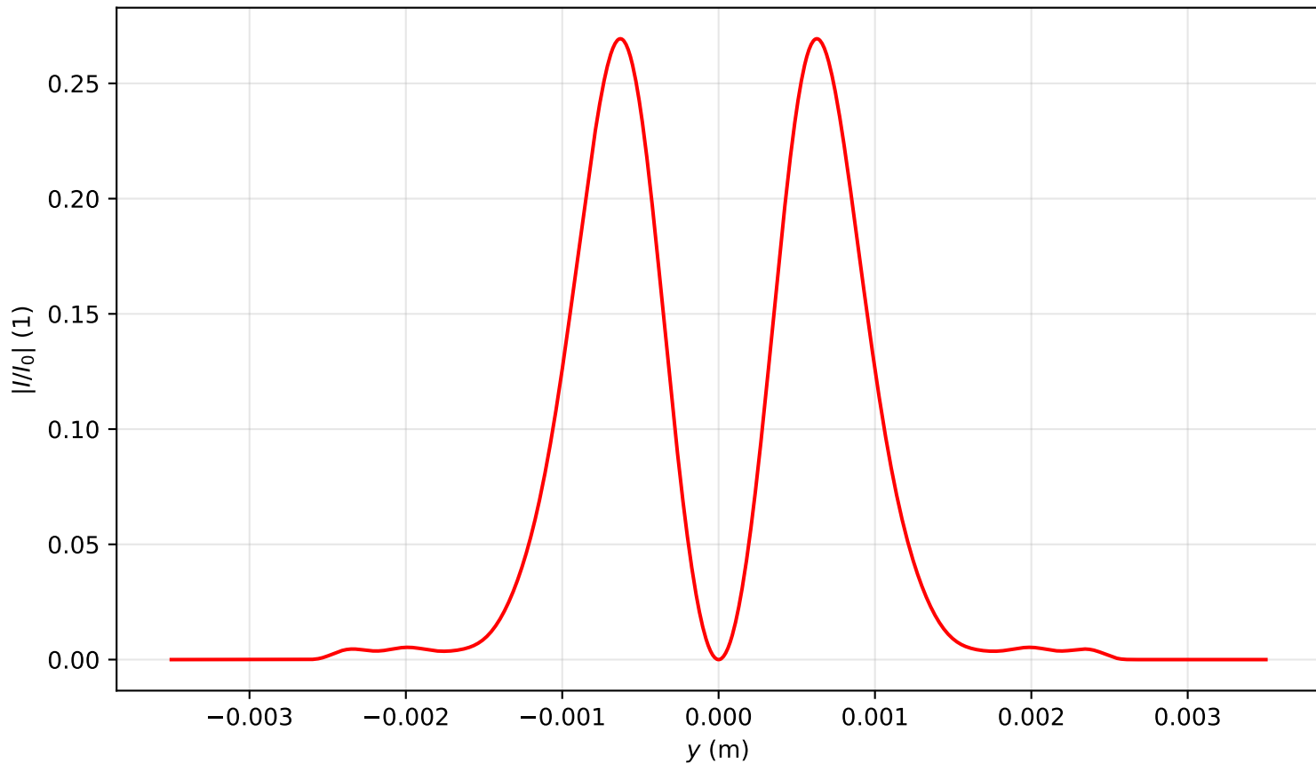
Intensity profile I(x=0, y, z=2.309)/I_0 , P_{in}=4.0P_{cr} , artificial time
